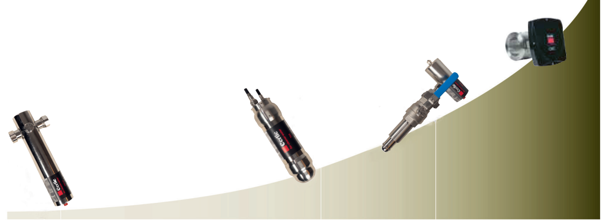
TSS-LC 10 mg/l TSS 10 000 mg/l TSS-IL 50 000 mg/l 5% CMC 300 000 mg/l 30%
